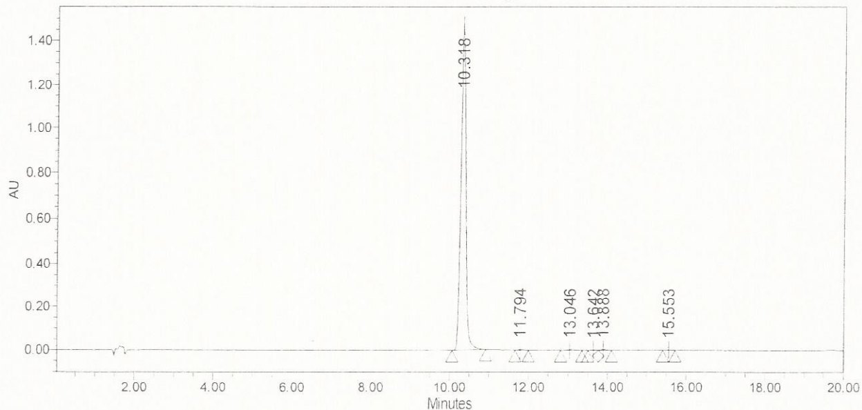
Auto-Scaled Chromatogram
